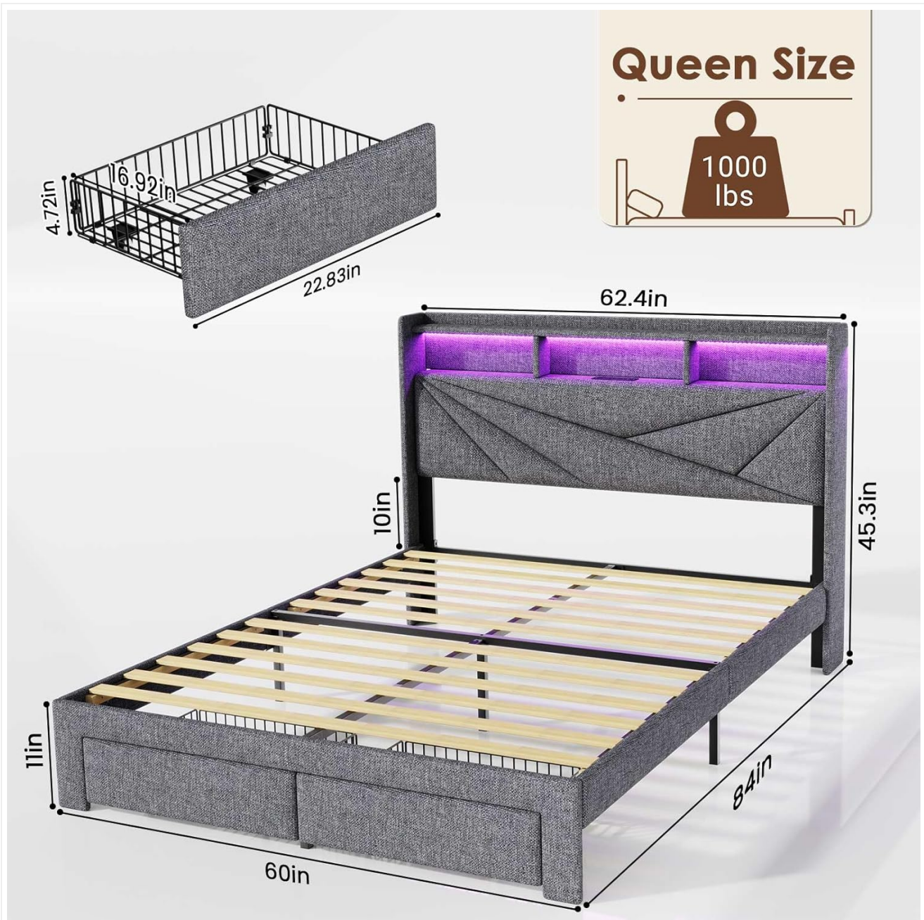
Image: An exploded view diagram illustrating the various components of the bed frame, including the headboard, frame, wooden slats, and storage drawers, along with key dimensions and the 1000 lbs weight capacity.
