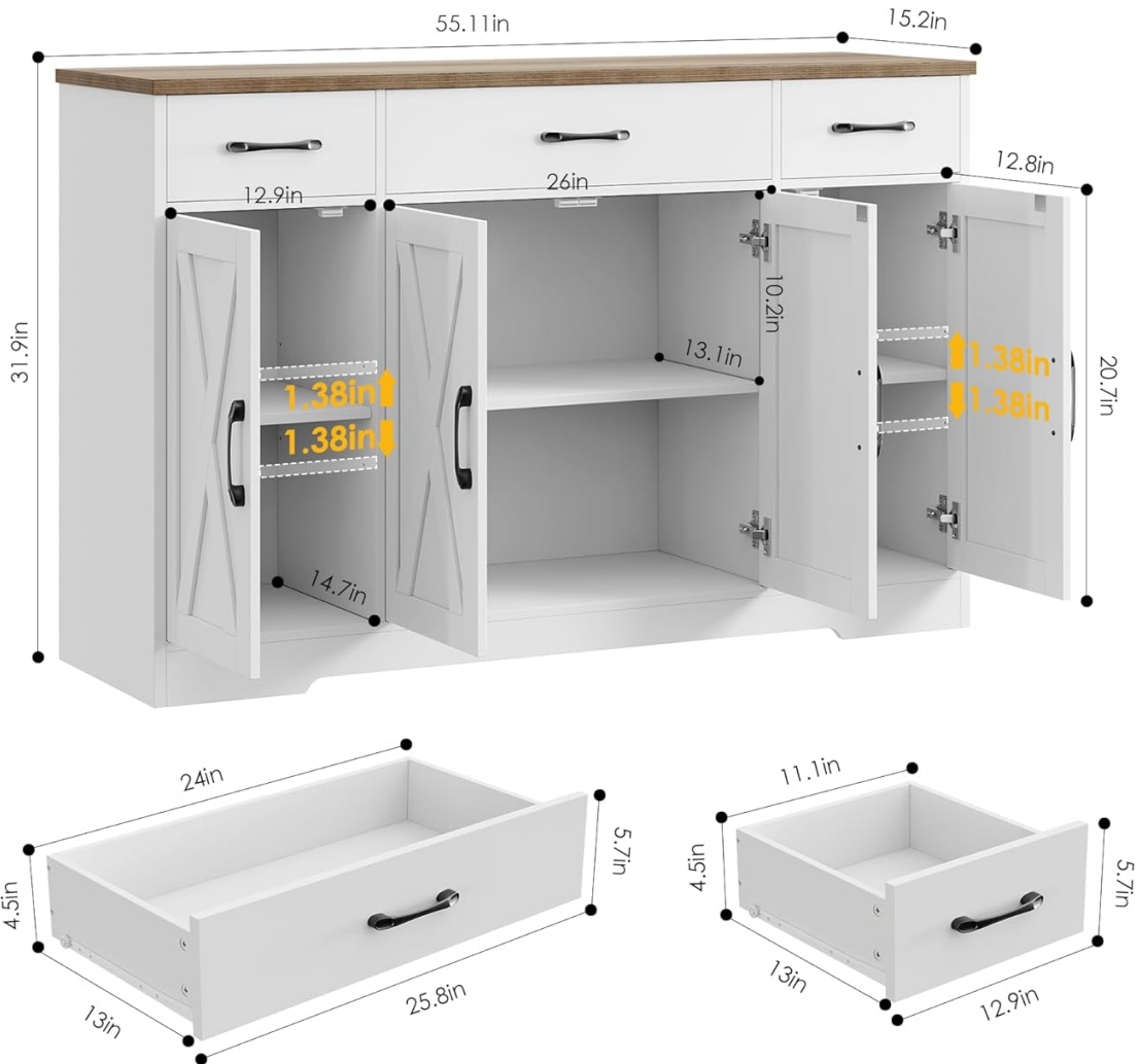
Image: Technical diagram showing product dimensions and weight capacities for various parts of the cabinet.
