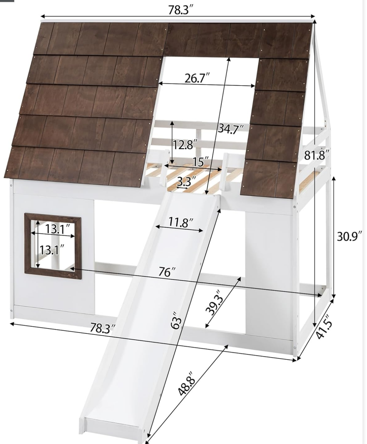
Figure 2: Dimensional drawing of the Polibi Bunk Bed. This diagram provides key measurements for the bed's length, width, height, and specific dimensions of the roof, window, ladder, and slide components, crucial for planning space and assembly.
