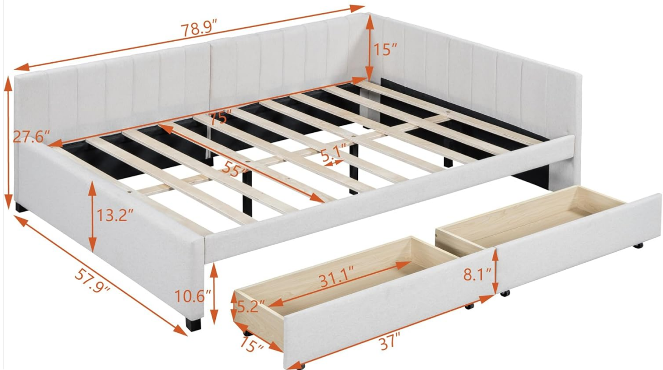
Image 1: Overall dimensions of the Merax Full Size Daybed, showing length, width, and height measurements for the frame and storage drawers.
