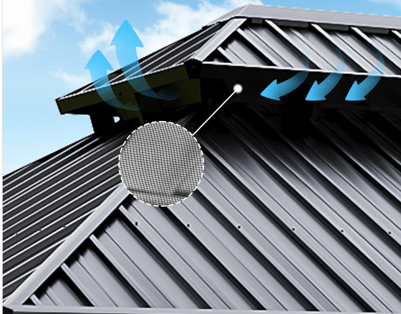
Image: The galvanized steel roof features a ventilated design for continuous air circulation.
