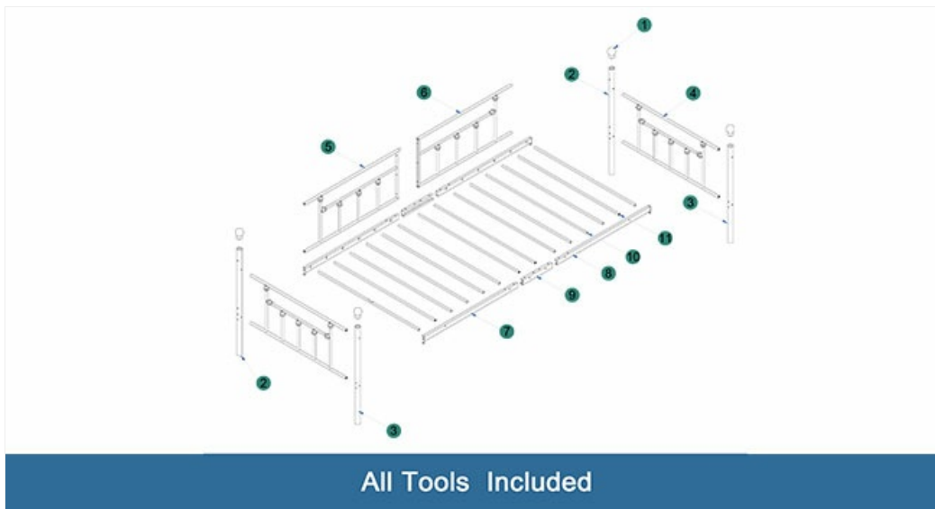
Figure 5.2: Unique Design Elements of the Daybed Frame.
