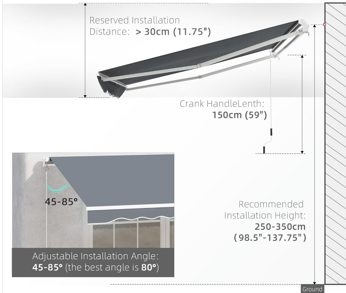
Figure 2: Recommended installation dimensions and adjustable angle (45-85 degrees, best at 80 degrees).
