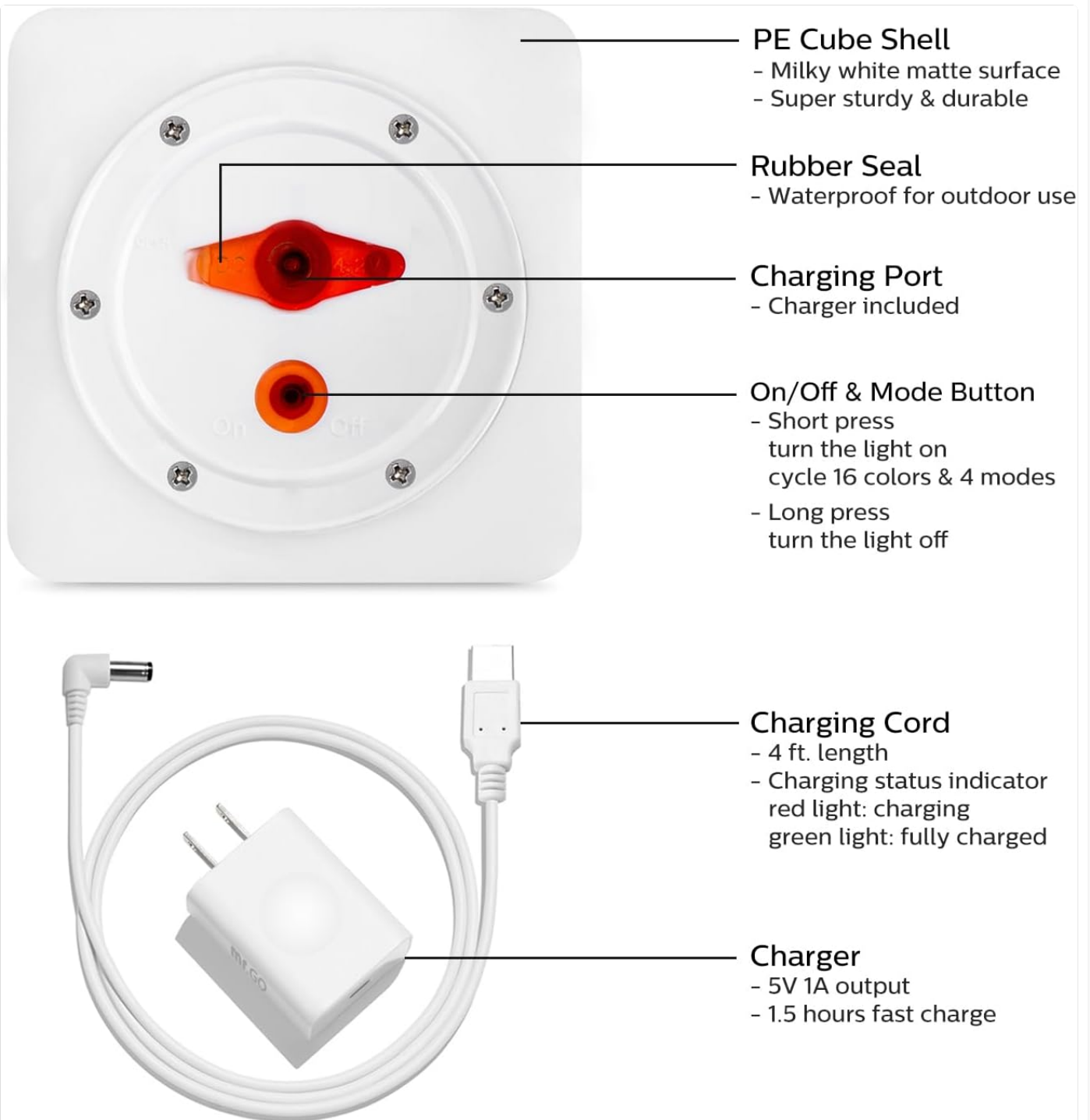
Image: A close-up view of the underside of the LED cube light, highlighting the PE cube shell, rubber seal, charging port, and the On/Off & Mode button.
