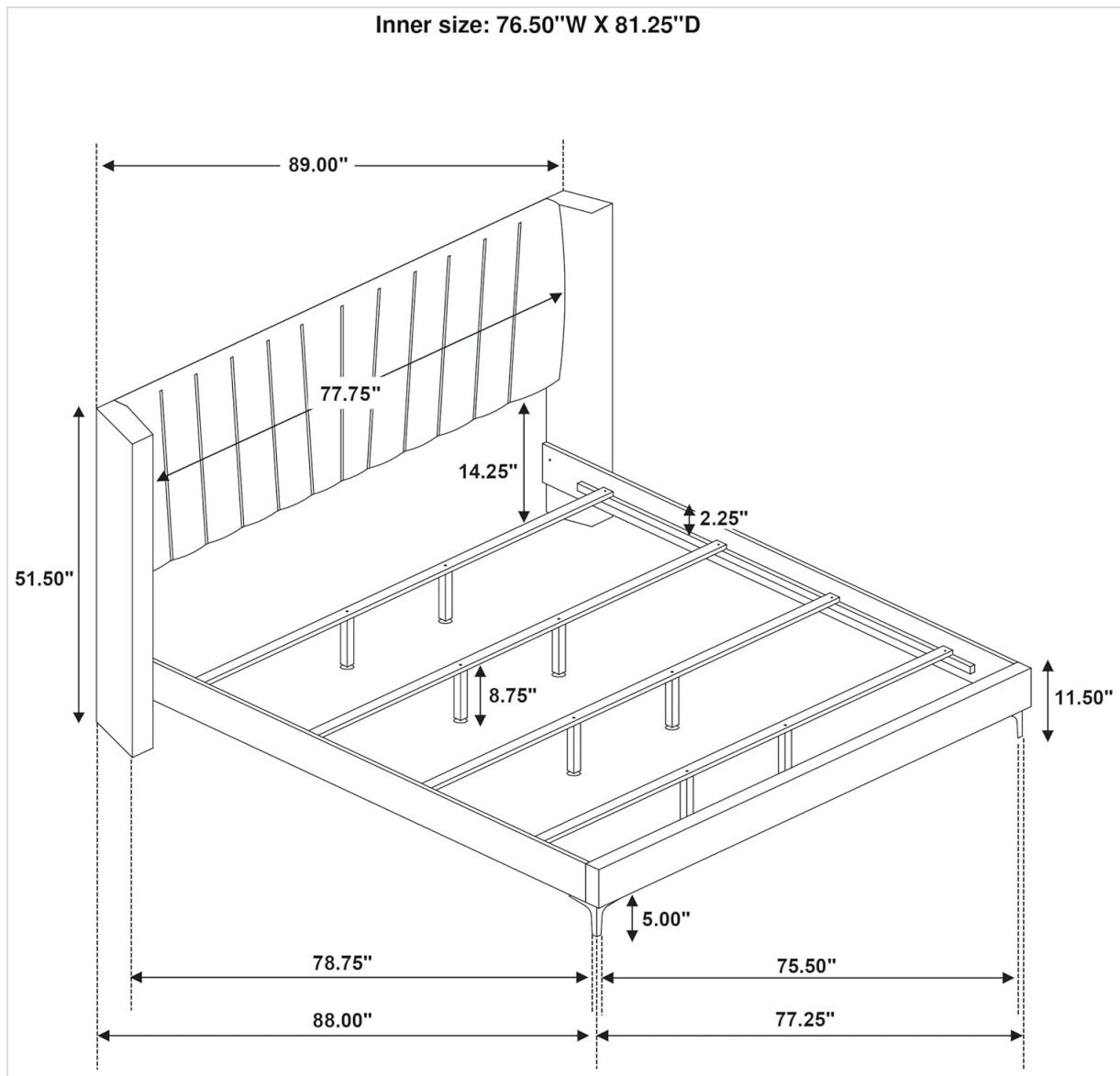
Image: Technical diagram illustrating the dimensions of the Coaster Kendall Eastern King Upholstered Bed, including length, width, and height measurements.
