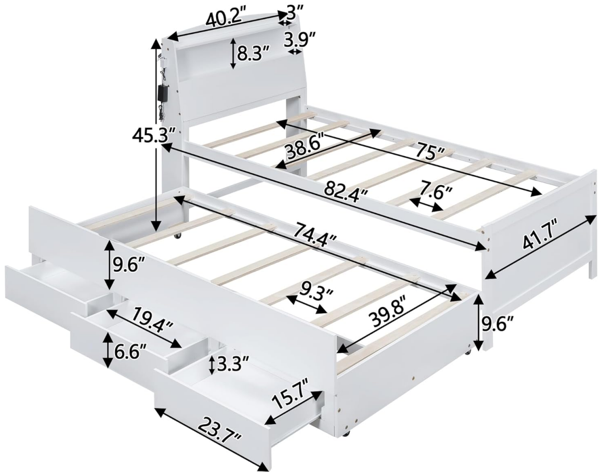
Image: Technical diagram illustrating the overall dimensions and key measurements of the Flieks Twin Platform Bed.
