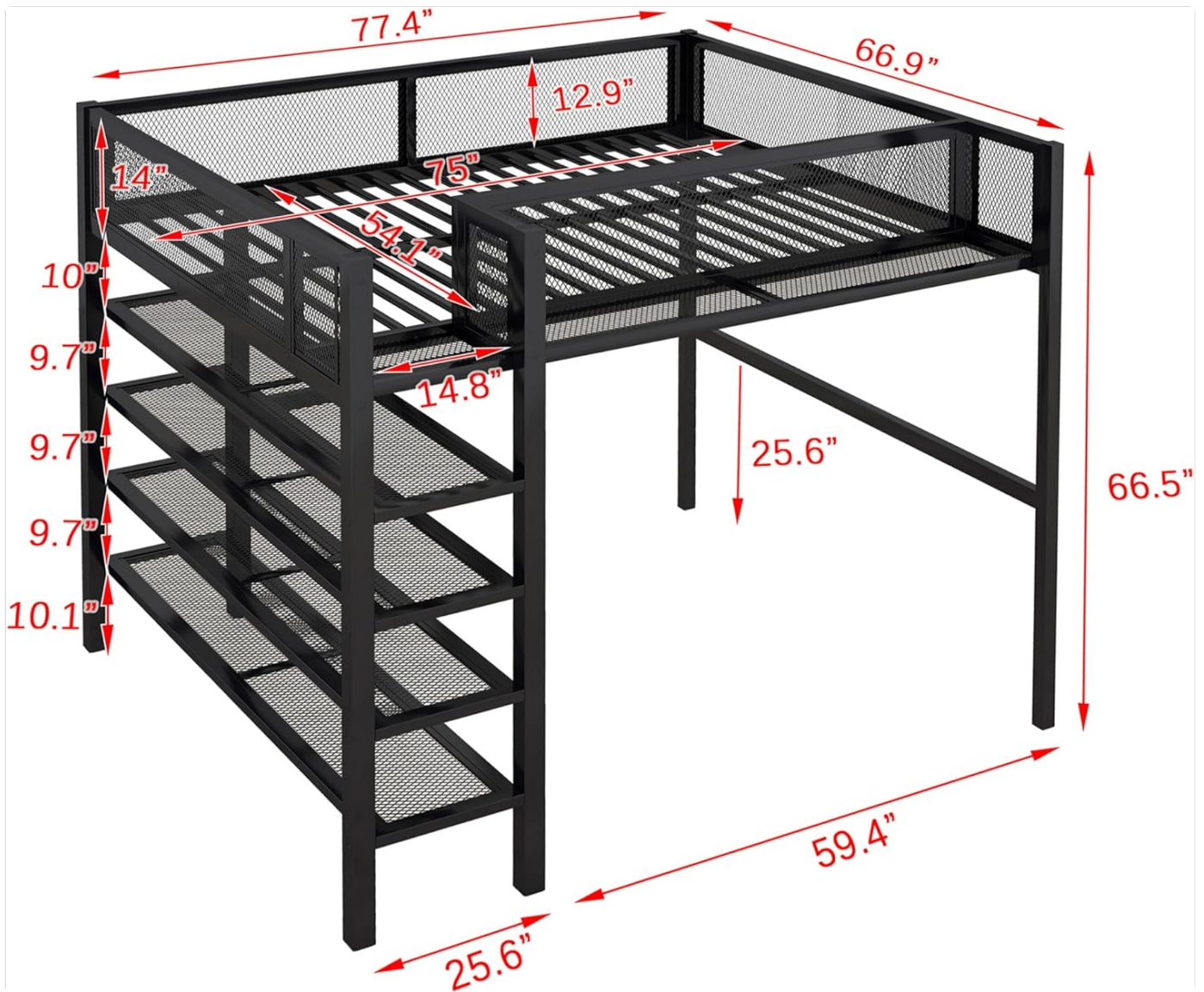
Image: A detailed diagram illustrating the precise dimensions of the Harper & Bright Designs Full Size Metal Loft Bed, including length, width, and height measurements for all key components.
