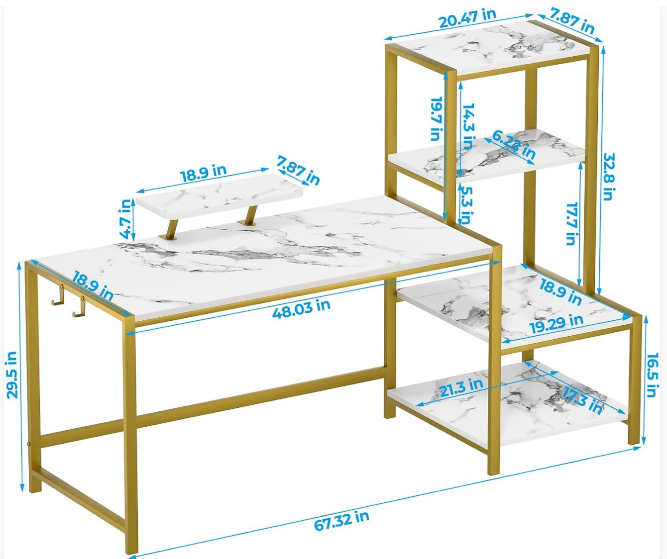
Image 2: Detailed dimensions of the desk, including the main desktop, printer shelf, and monitor stand.
