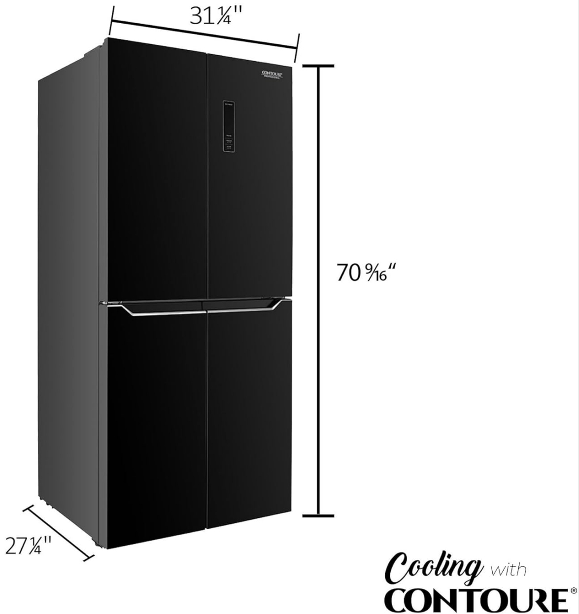
Figure 1: Refrigerator Dimensions. This image illustrates the overall dimensions of the CONTOURE RV Deluxe Refrigerator, showing a width of 31 1/4 inches, a depth of 27 1/4 inches, and a height of 70 9/16 inches. These measurements are crucial for proper placement and installation.
