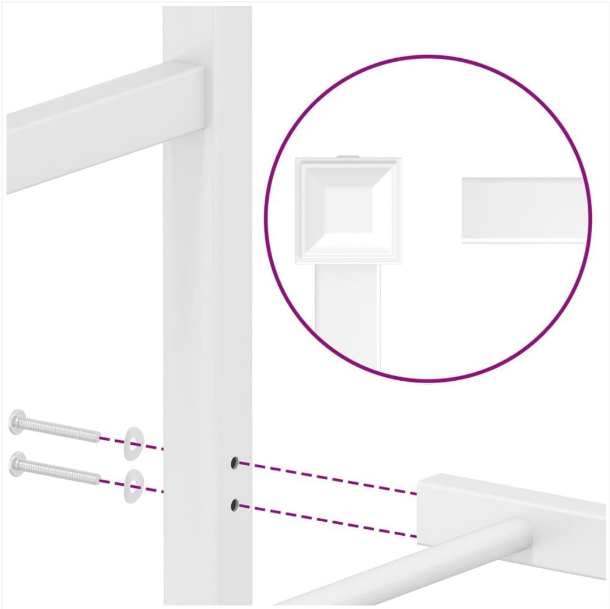
Image: Illustration demonstrating the connection method for bed frame components using bolts.
