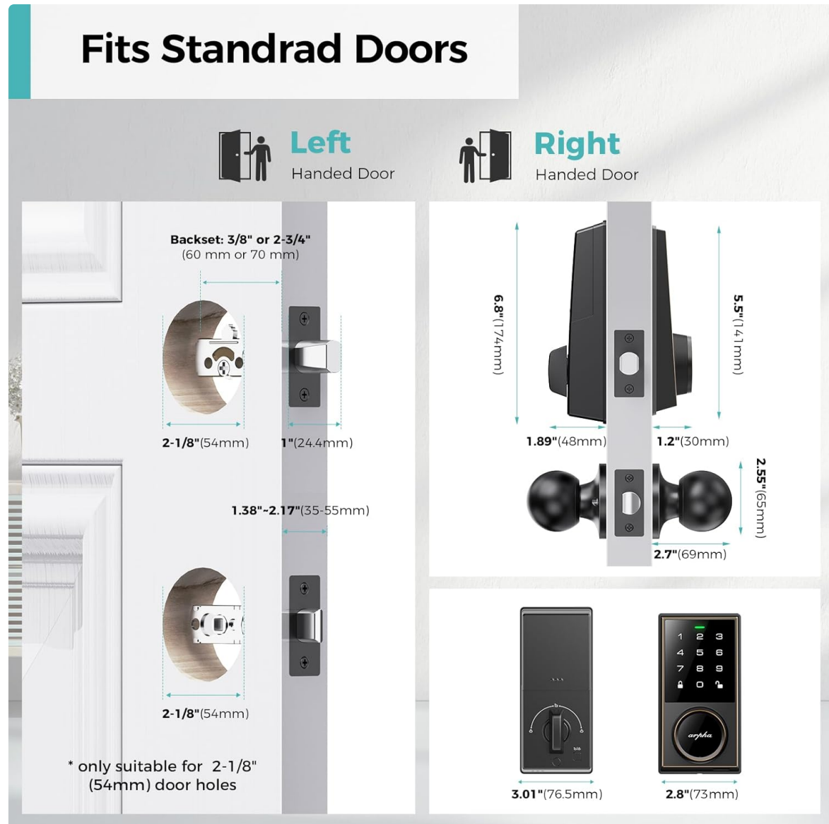
Figure 3: Door Compatibility and Dimensions
