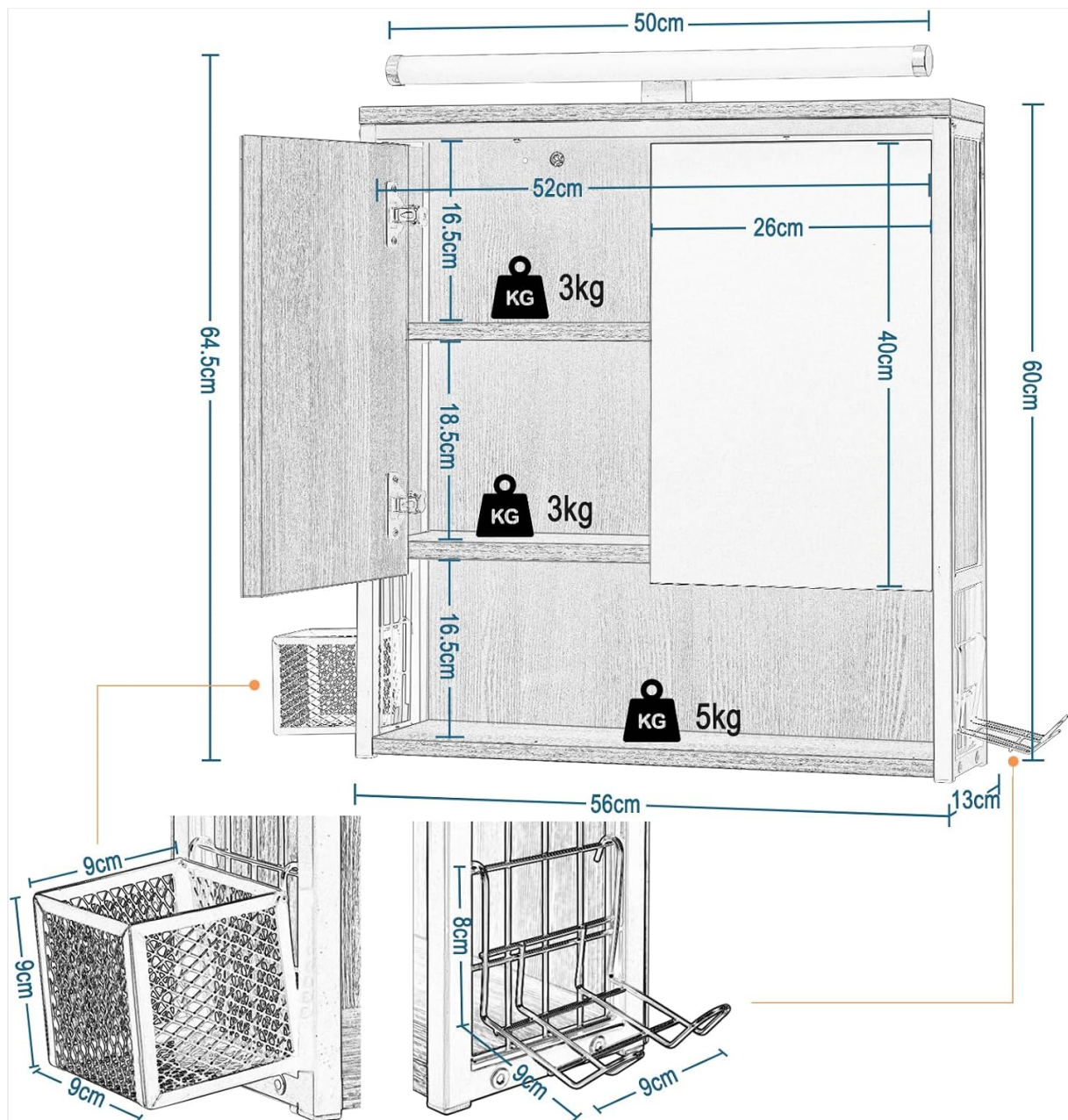
Figure 2: Product Dimensions and Load Capacities. Note: Internal shelves support 3kg each, bottom shelf 5kg.
