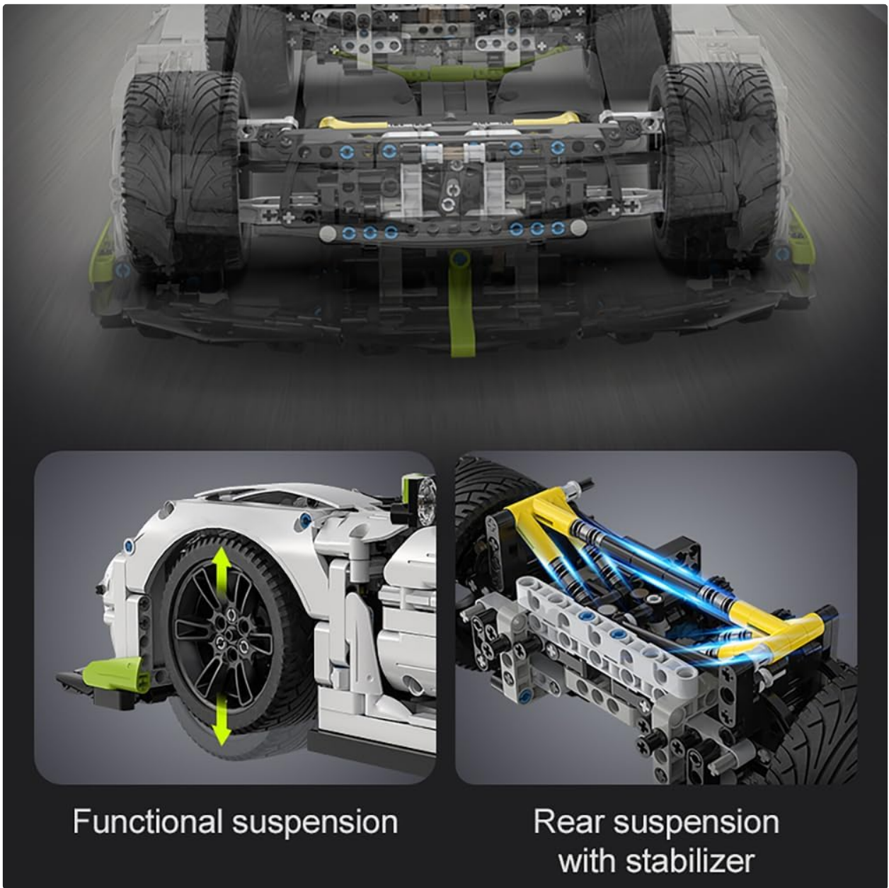
Image: Two views of the CaDA Fantasma model's suspension system: a demonstration of the functional suspension and a detailed look at the rear suspension assembly, including its stabilizer components.
