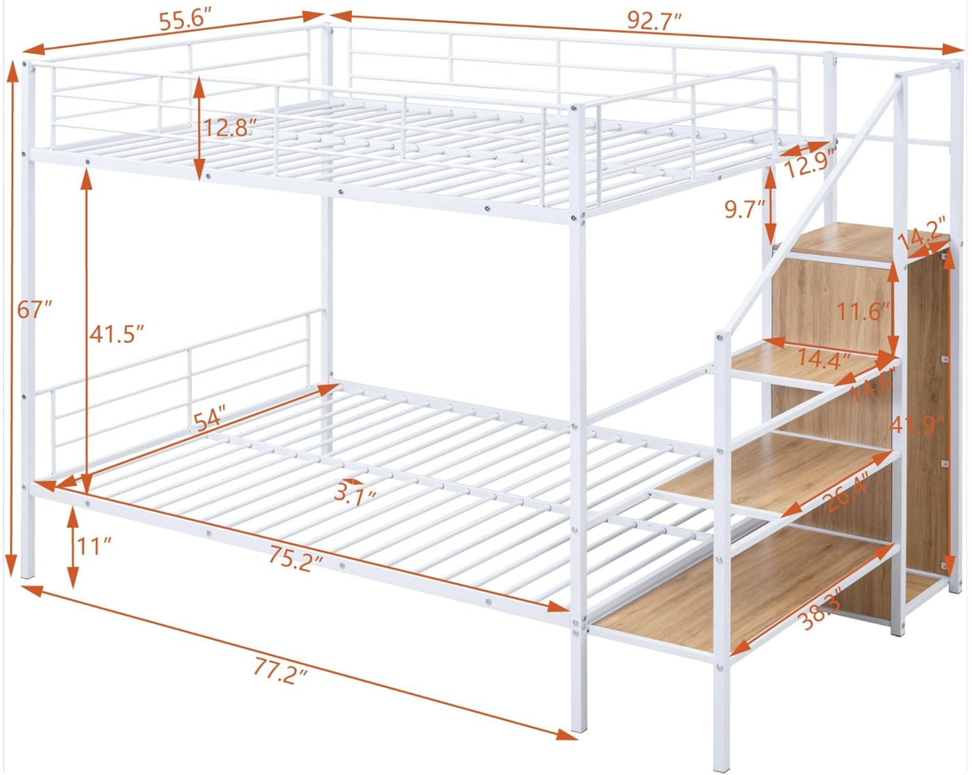
Image: Diagram showing the detailed dimensions of the Fliexs Full Over Full Metal Bunk Bed in inches.
