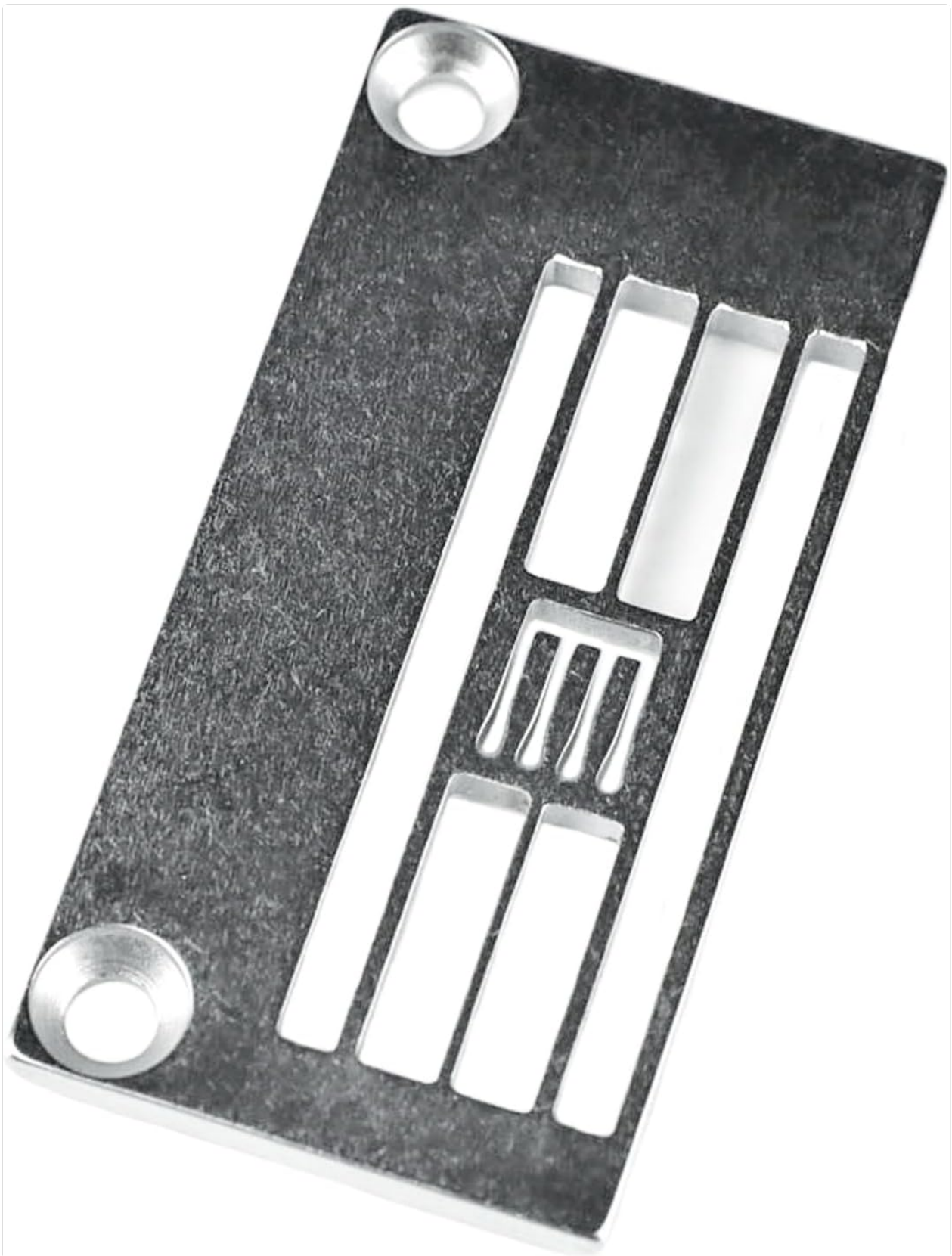
Figure 1.1: Top view of the Blooy E1828 Throat Plate, showing the needle slots and feed dog openings.
