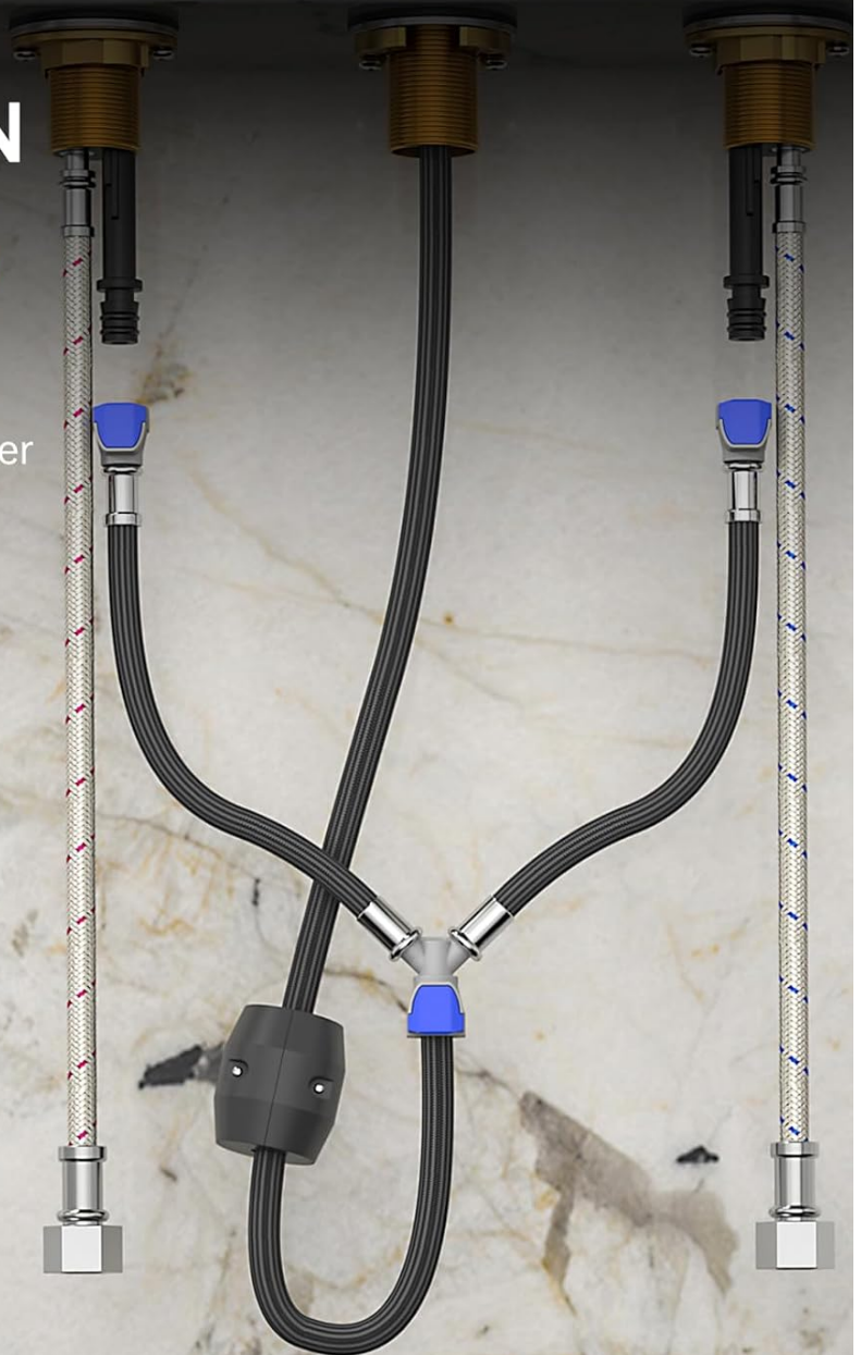
Figure 4: Illustration of the wrench-free quick-connect hose system for simplified installation.
