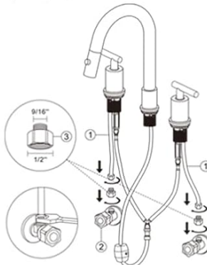
Figure 3: Comprehensive step-by-step installation diagram for the faucet, handles, and water connections.
