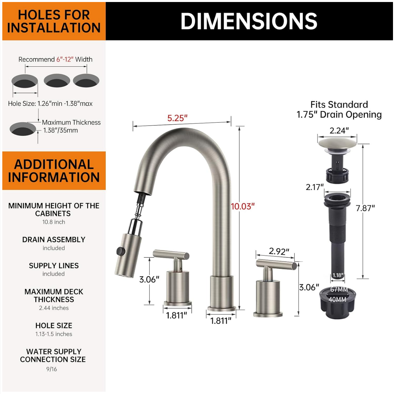
Figure 2: Detailed dimensions of the faucet and handles, along with recommended hole sizes and spacing for installation on a 3-hole widespread sink (6-12 inch width).
