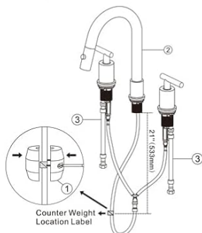
Figure 3: Comprehensive step-by-step installation diagram for the faucet, handles, and water connections.
