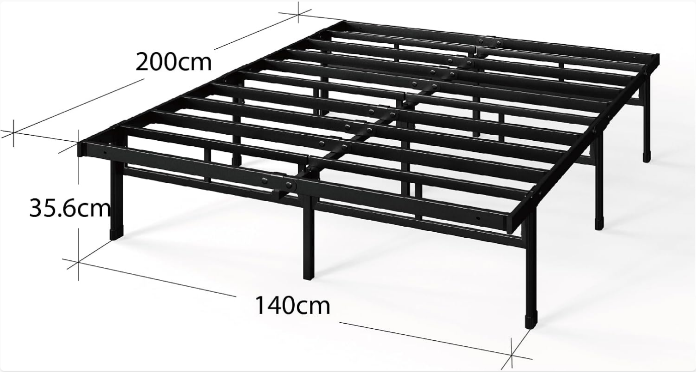
Figure 8: Product Dimensions
