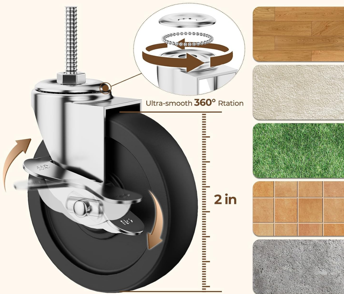
Figure 5.1: Detail of the silent and lockable wheels.
