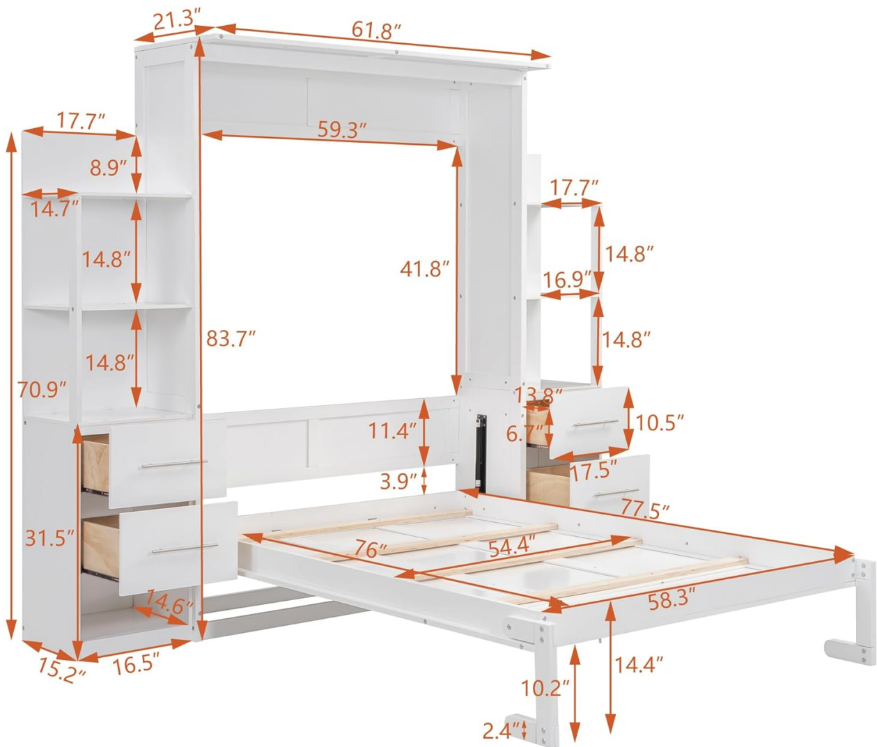
Figure 7: Detailed dimensions of the KLMM Full Size Murphy Bed in both open and closed configurations.
