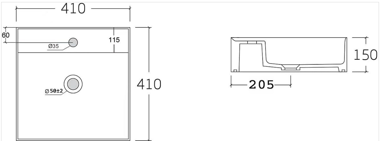
Image: Technical drawing illustrating the dimensions of the VERINI square countertop basin, including length, depth, height, and diameters for faucet and drain holes.
