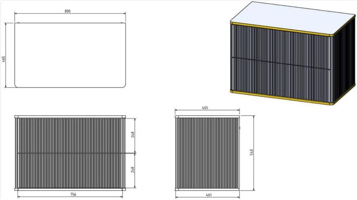
Figure 4: Technical drawing illustrating the dimensions of the KELIZA vanity unit.
