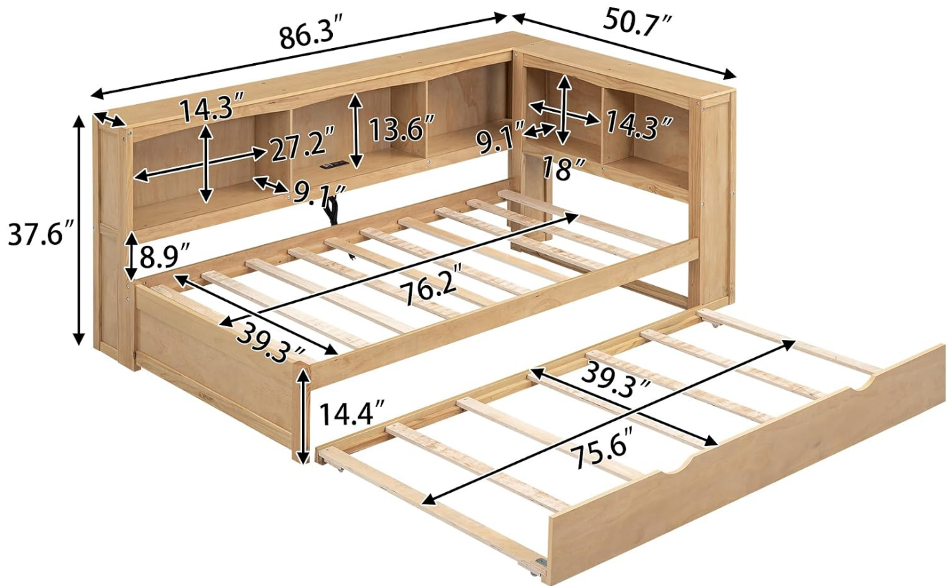
Detailed dimensions of the Brabrety Twin Size Daybed, including length, width, height, and trundle measurements.
