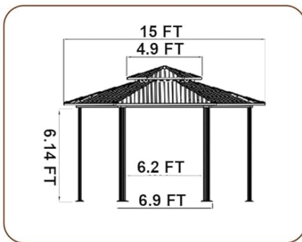
Image 4.1: Dimensional drawing of the 15x15FT Hexagon Hardtop Gazebo, providing key measurements for planning and installation.
