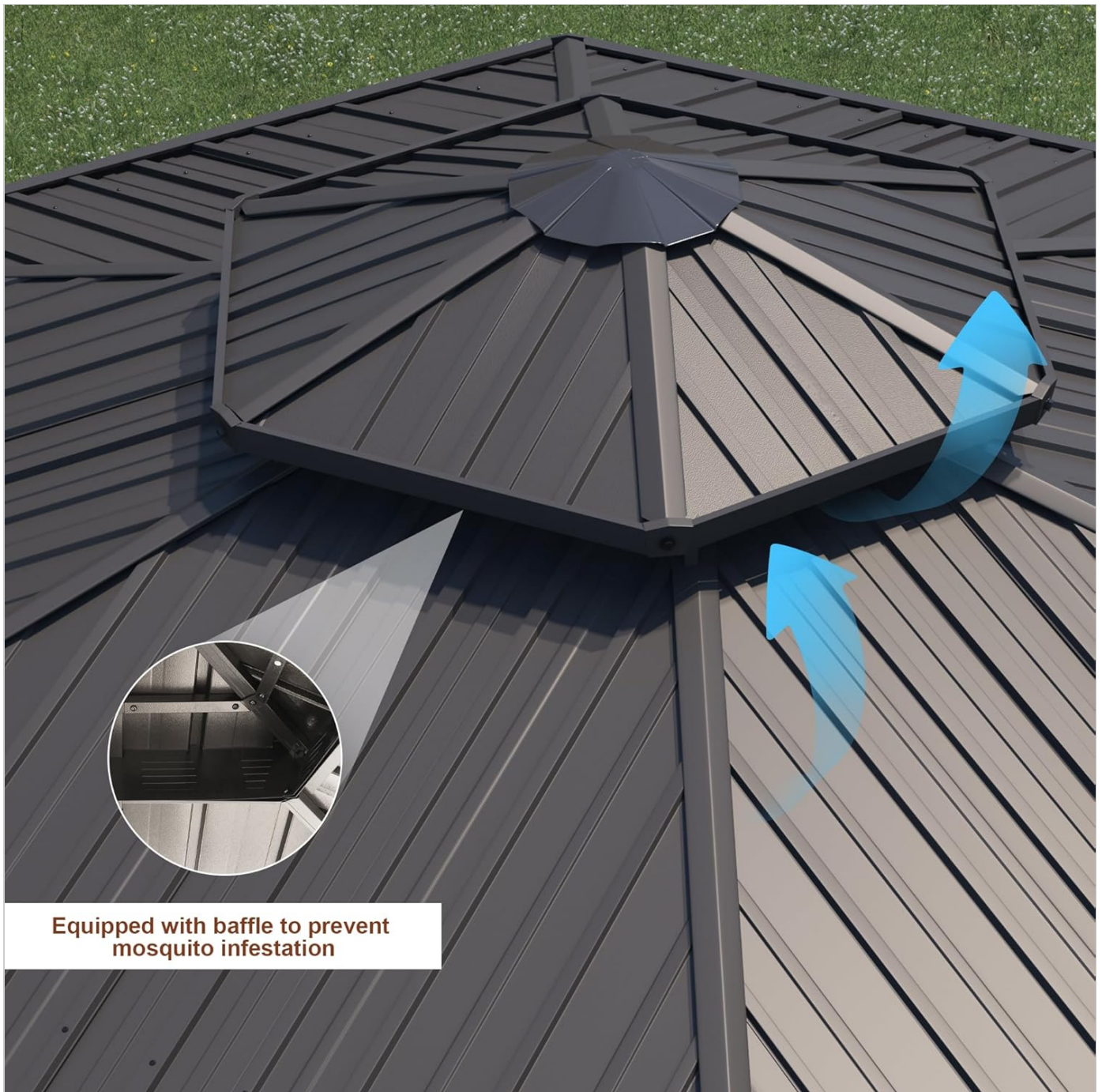
Image 3.2: The double roof design with arrows illustrating optimal airflow and a close-up of the integrated baffle for mosquito prevention. The roof's sloping design ensures efficient drainage, preventing rainwater accumulation and extending the product's service life.
