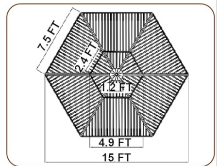
Image 4.1: Dimensional drawing of the 15x15FT Hexagon Hardtop Gazebo, providing key measurements for planning and installation.
