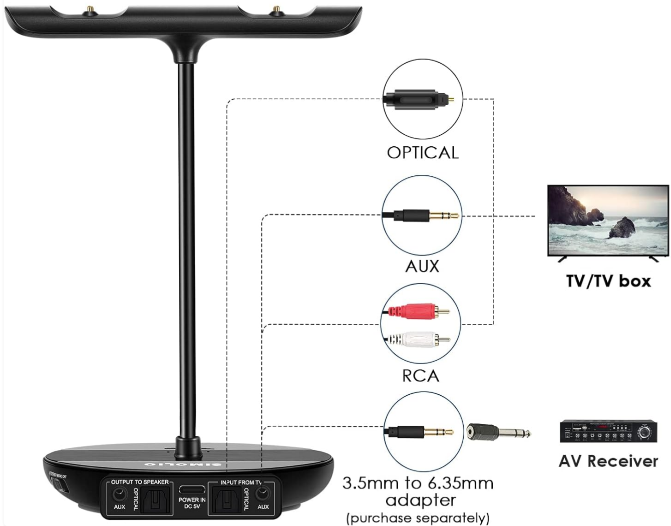
Image: A diagram illustrating the various audio input options for the transmitter, including Optical, AUX, and RCA connections to a TV or AV Receiver.
