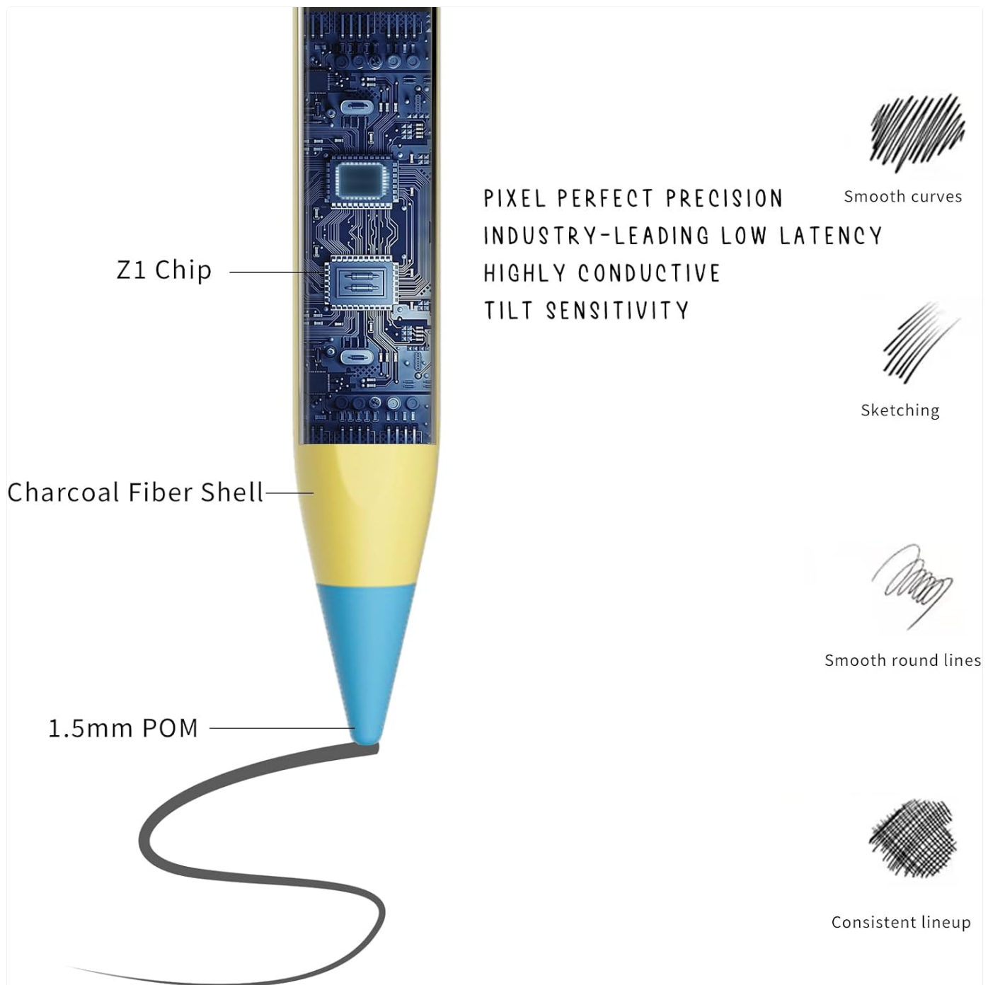
Figure 3: Detailed view of the stylus pen's internal Z1 chip, charcoal fiber shell, and 1.5mm POM tip, highlighting pixel-perfect precision and tilt sensitivity for various drawing styles.
