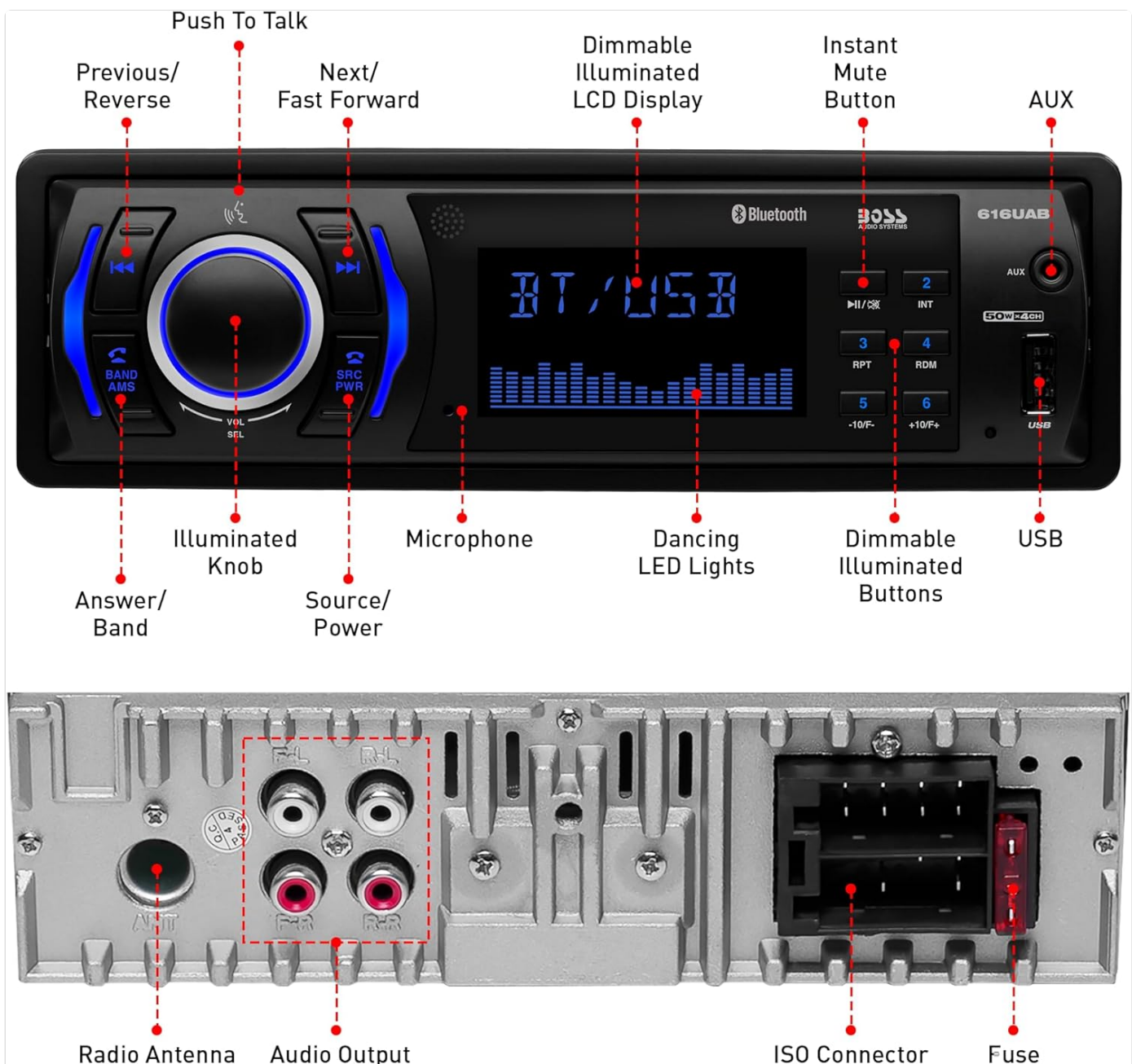
Figure 5: Front panel controls of the 616UAB receiver. Key controls include Answer/Band, Previous/Reverse, Push To Talk, Illuminated Knob (Volume/Select), Source/Power, Microphone, Dancing LED Lights, Dimmable Illuminated Buttons, Instant Mute Button, AUX input, and USB port.
