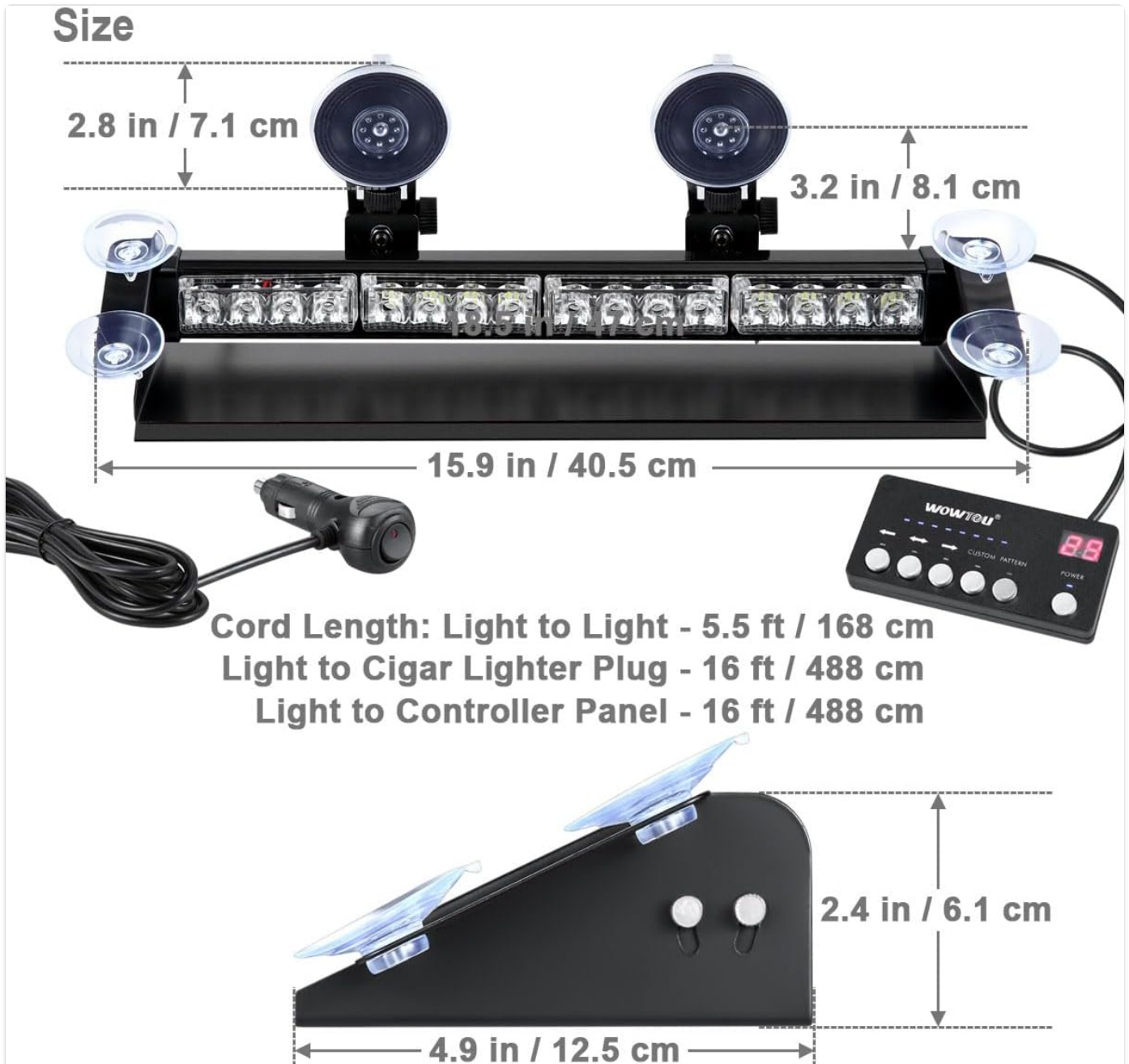
Figure 5: Visual guide for both windshield and L-bracket mounting methods.
