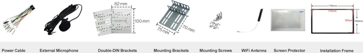
Figure 1: Package Contents and Double DIN Dimensions. This image illustrates the items included in the product package and provides dimensional specifications for the double DIN unit, showing its compatibility with standard dash kits.
