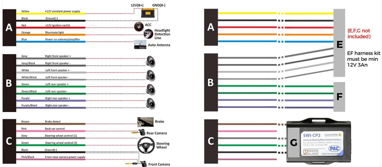
Double DIN dimensions and wiring diagram for installation.
