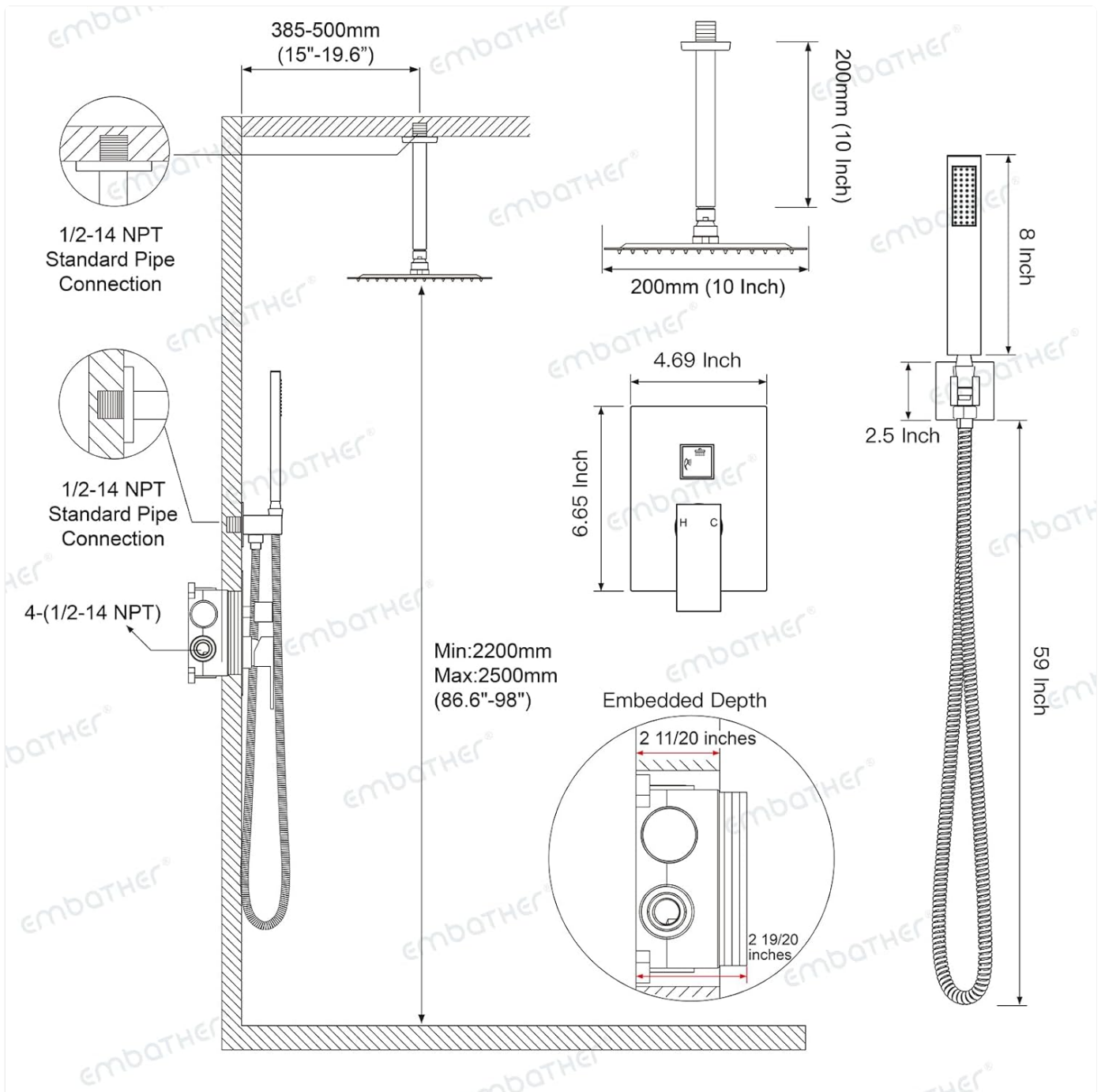
Figure 3.2: Technical drawing illustrating the dimensions and installation points for the shower system components.
