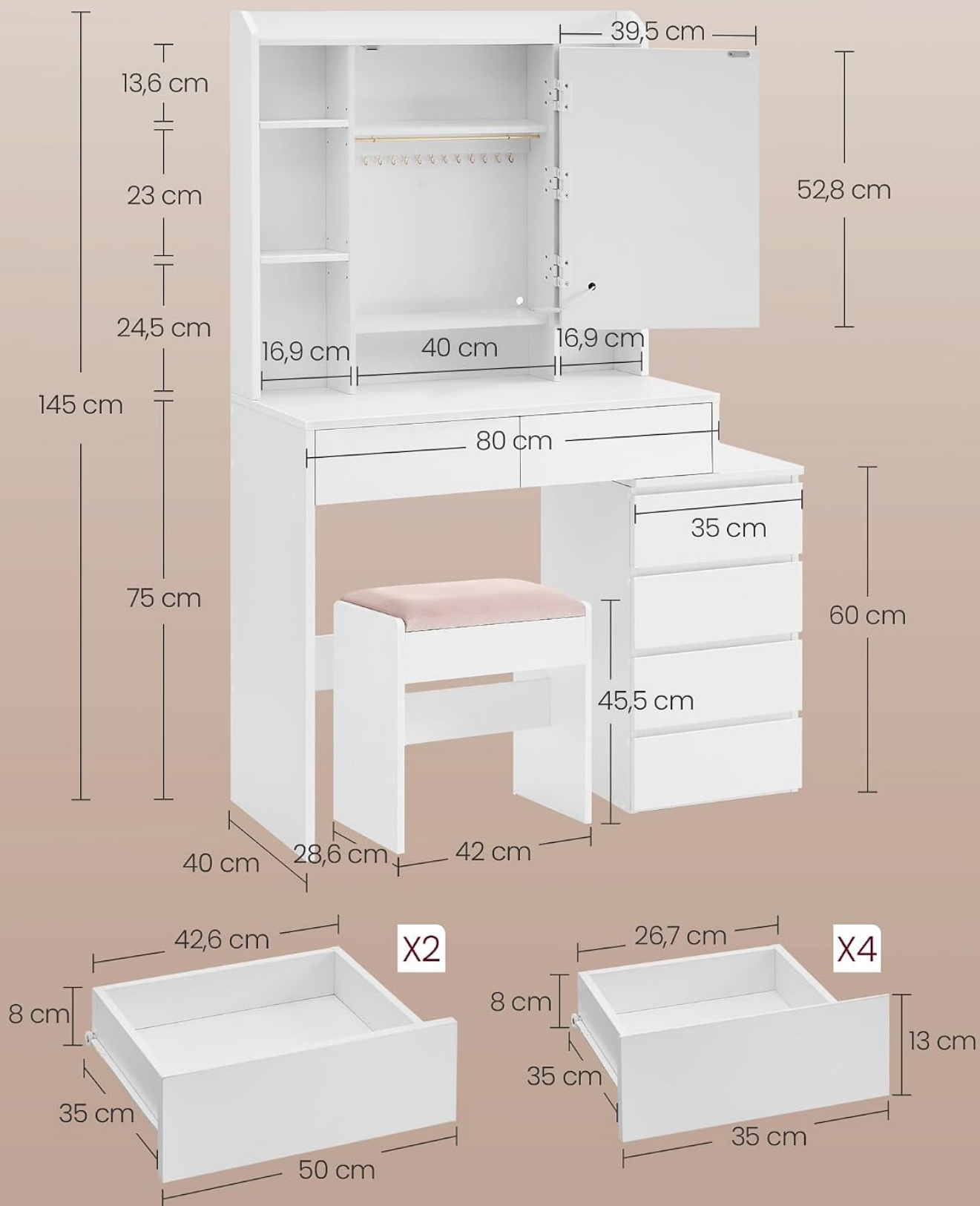
Image 4.1: Detailed dimensions of the dressing table and its components, including drawer sizes, to assist with planning and assembly.
