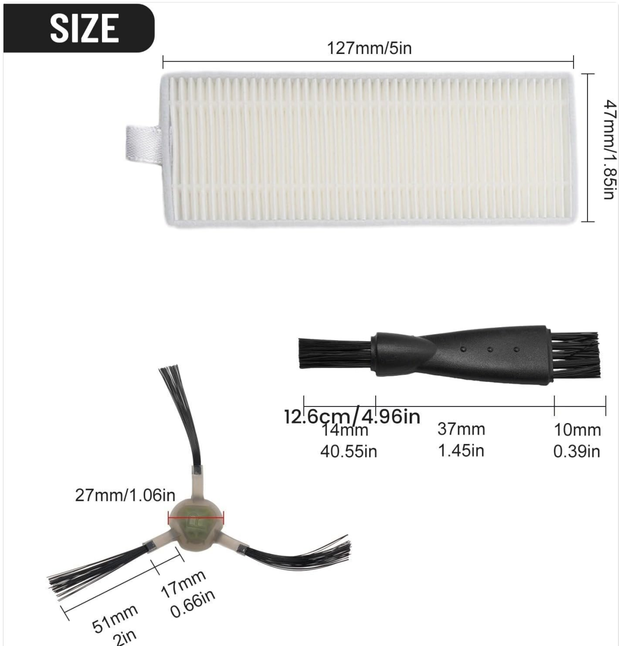
Image 6.1: Visual representation of the approximate dimensions for both the replacement filter and side brush.
