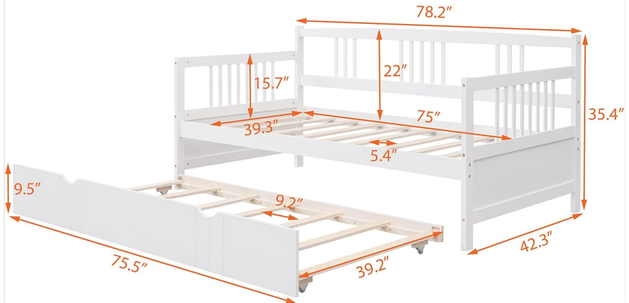
Image 8.1: Detailed dimensions of the Fliex Daybed and its trundle component.
