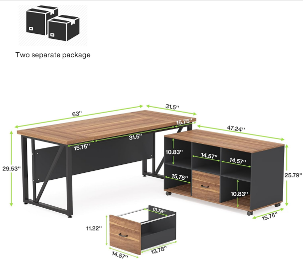
Figure 2: Detailed dimensions of the desk and mobile file cabinet, indicating two separate packages for delivery.
