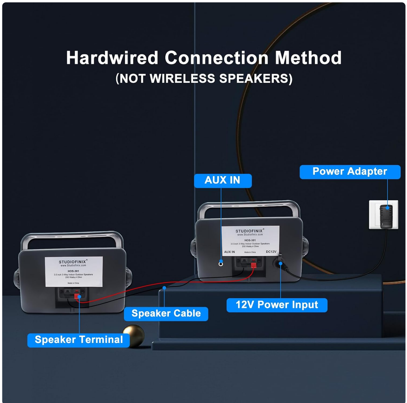
Image: Hardwired connection diagram for the STUDIOFINIX speakers.
