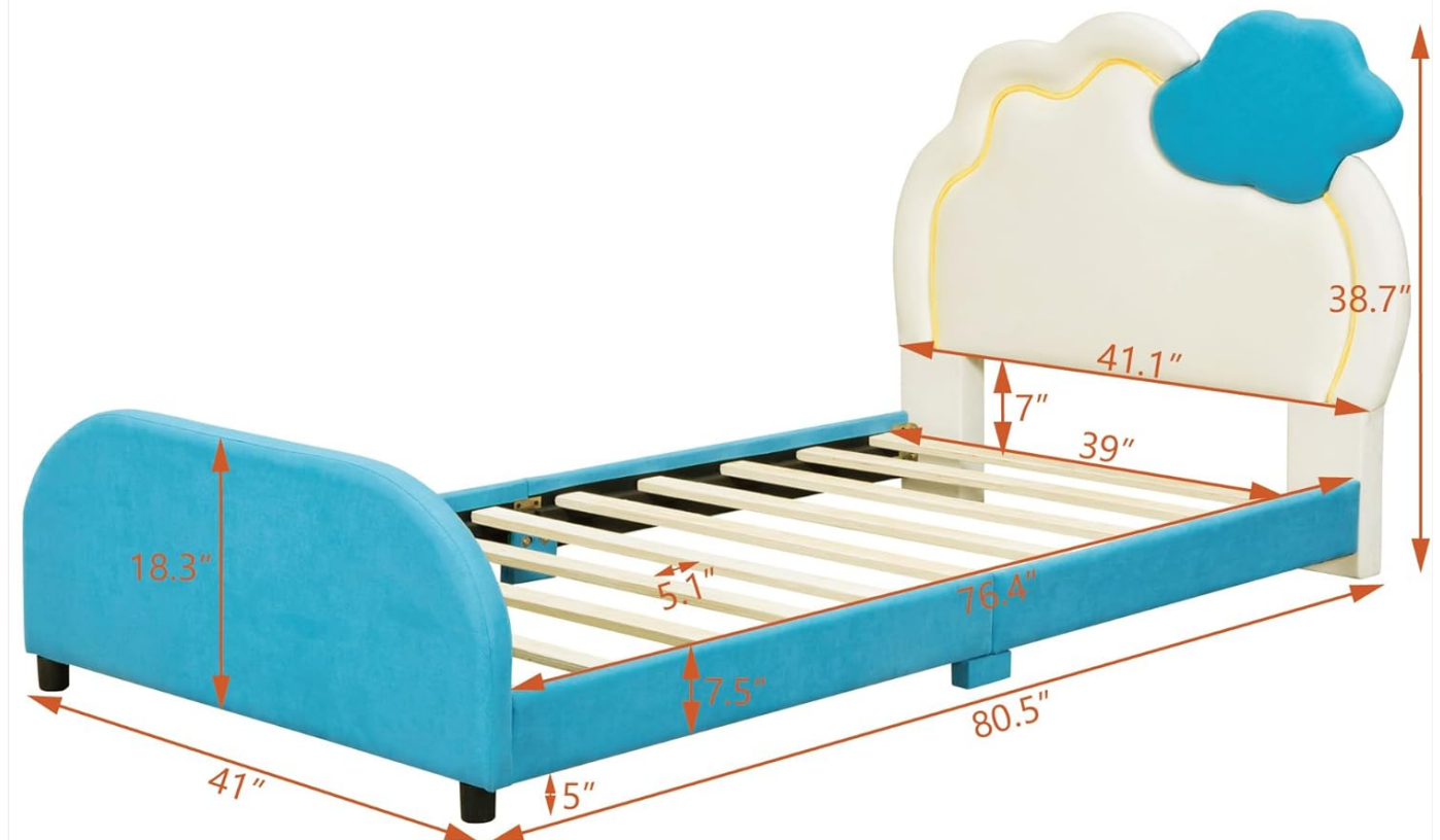
Figure 3.1: Overall dimensions of the bed frame. Length: 80.5", Width: 41", Headboard Height: 38.7", Footboard Height: 18.3", Ground Clearance: 5".
