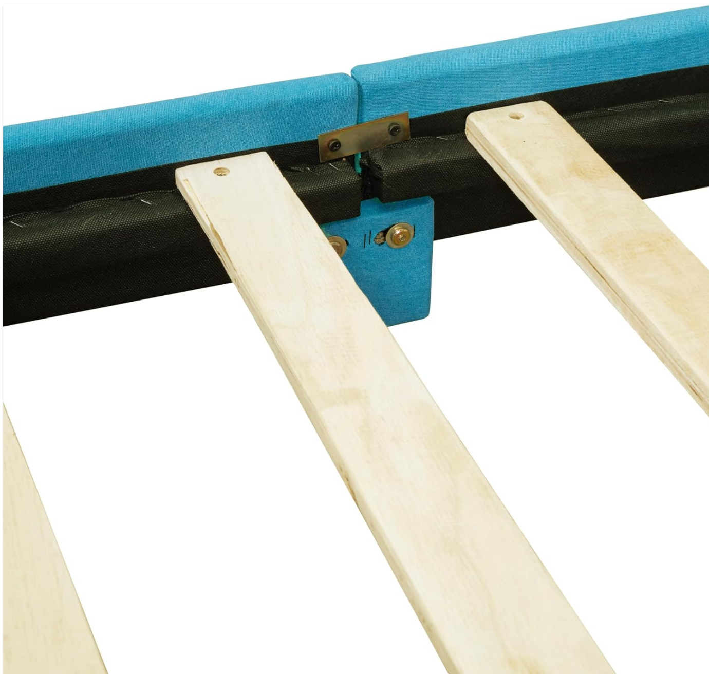
Figure 4.4: Detail of the wooden bed slats and the central support mechanism, ensuring mattress stability.
