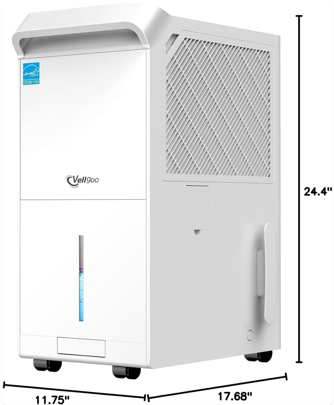
Figure 6: Dehumidifier Dimensions. This image provides a visual representation of the unit's dimensions: 17.68 inches deep, 11.75 inches wide, and 24.4 inches high.
