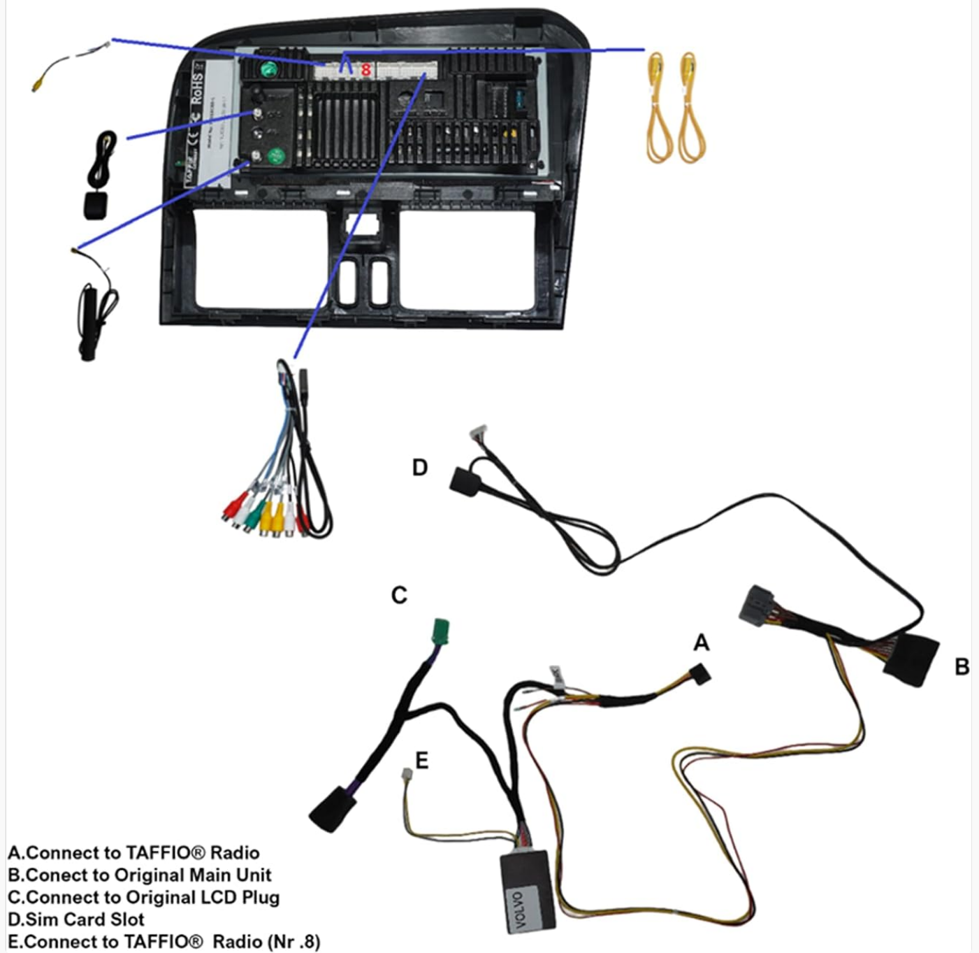
Figure 3.2.1: General installation diagram showing connection points for the Taffio system. A: Connect to Taffio Radio, B: Connect to Original Main Unit, C: Connect to Original LCD Plug, D: SIM Card Slot, E: Connect to Taffio Radio (Nr.8).
