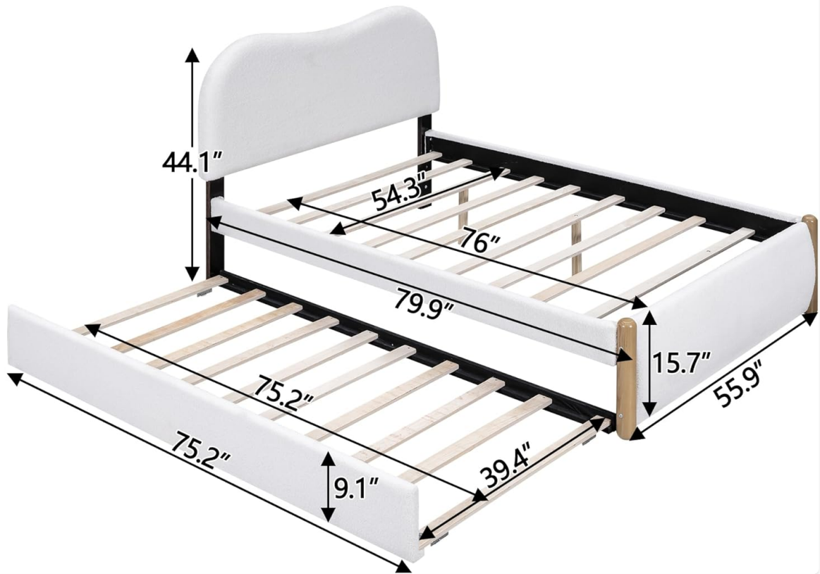
Image: Detailed diagram showing the dimensions of the Mirightone Full Bed Frame and its trundle.
