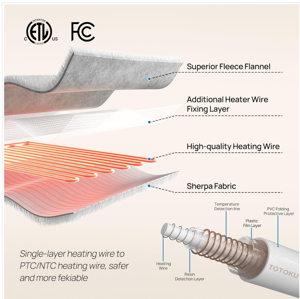
Figure 2: Cross-section diagram illustrating the multi-layered construction of the blanket, including superior fleece flannel, heater wire fixing layer, high-quality heating wire, and Sherpa fabric.
