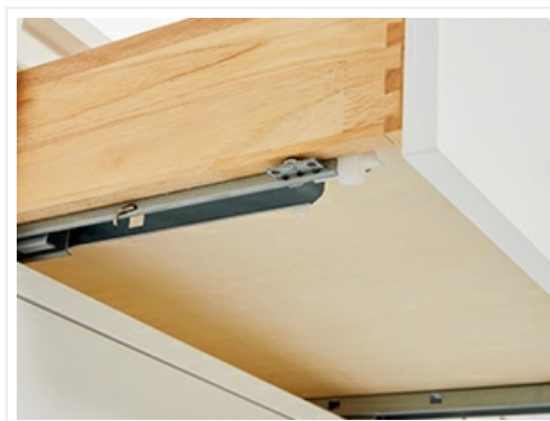
Figure 6: Detail of the soft-closing mechanism for doors and drawers.
