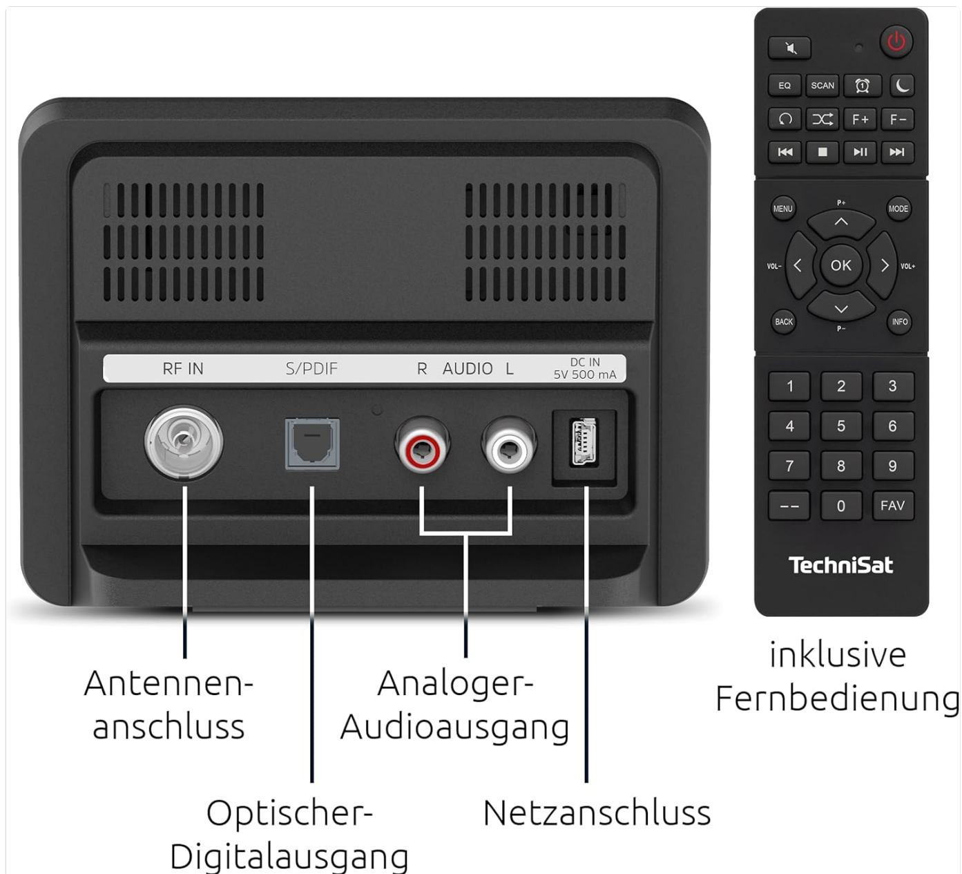
Image: Rear panel of the DIGITRADIO 11 IR, illustrating the antenna connection, optical digital output, analog audio output, and power input. The included remote control is also shown.
