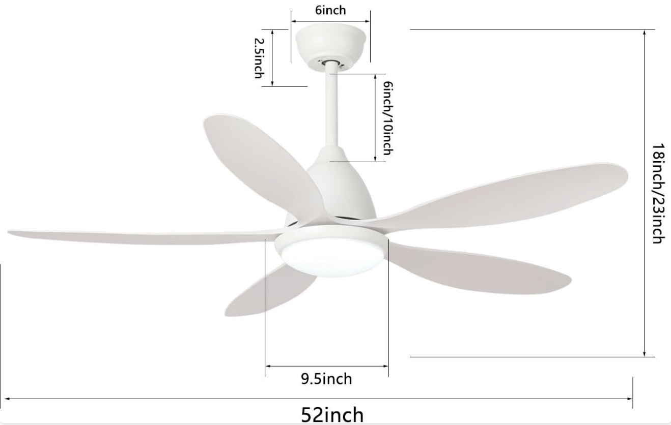
Figure 4.1: Detailed dimensions, installation types (flat and angled), and included downrods.
