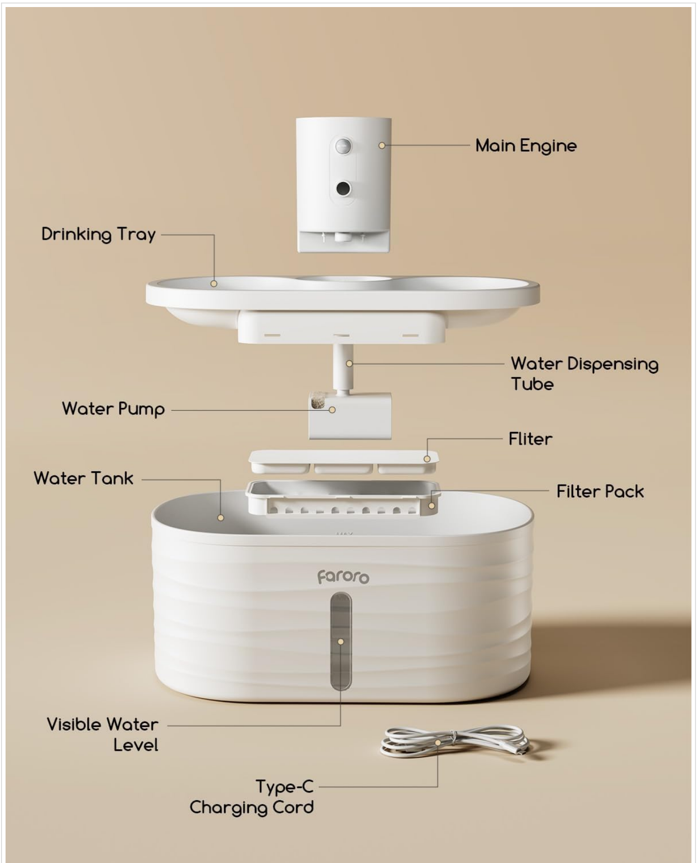
Image 2.1: Exploded diagram showing the main engine, drinking tray, water dispensing tube, water pump, filter, filter pack, water tank, visible water level indicator, and Type-C charging cord.
