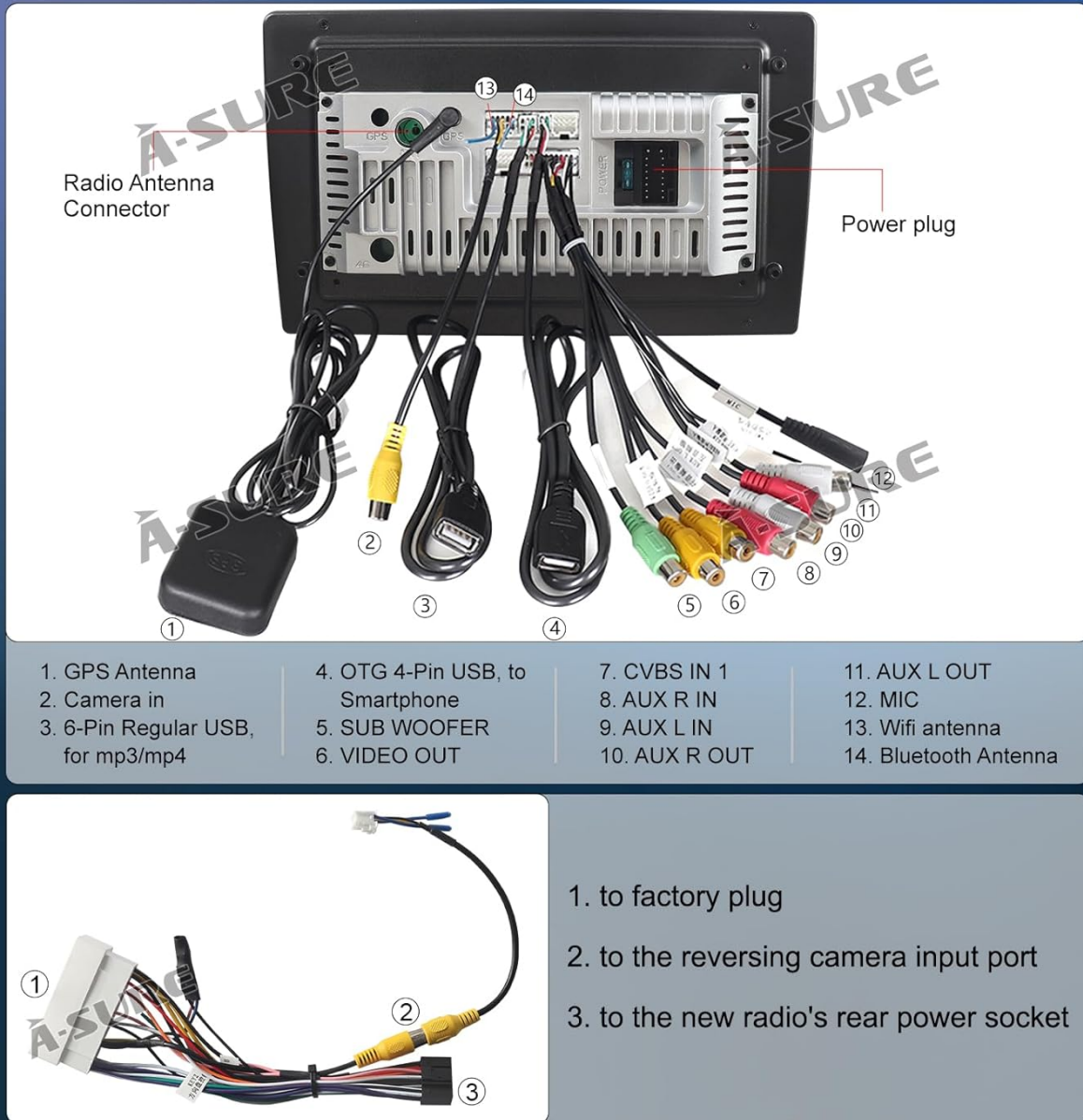
Figure 4.2: Ports illustration for connecting various components to the car stereo.
