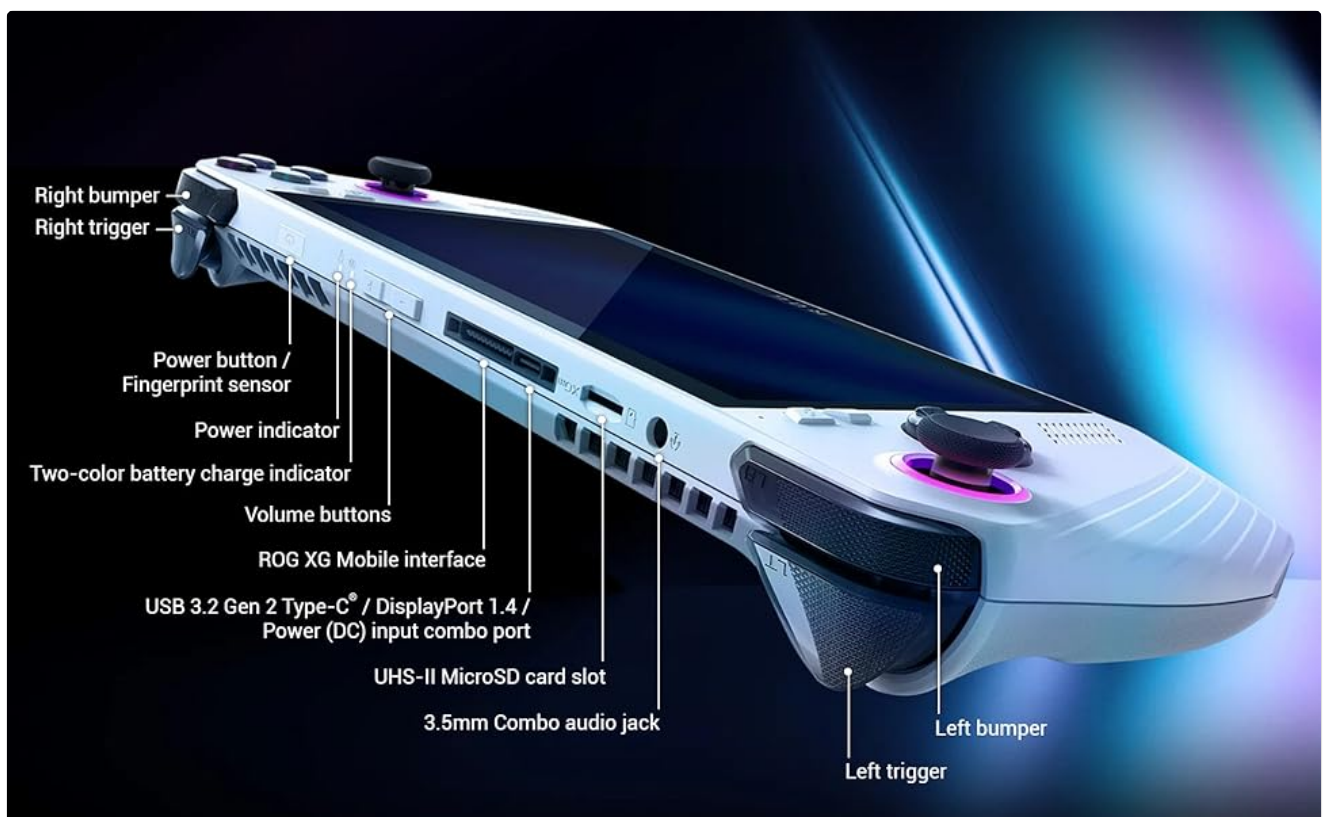
Figure 2.3: Side view of the ROG Ally showing the right bumper, right trigger, power button/fingerprint sensor, power indicator, two-color battery charge indicator, volume buttons, ROG XG Mobile interface, USB 3.2 Type-C / DisplayPort 1.4 / Power (DC) input combo port, UHS-II MicroSD card slot, and 3.5mm Combo audio jack.
